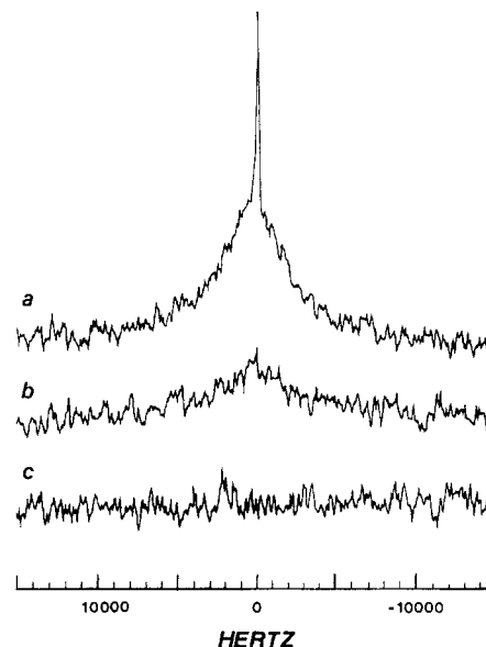
Figure 4. Solid-state ^2\text{H} -NMR spectra of PLG50:50 containing 1.17% ^2\text{H}_2\text{O} (a), the sample dried under vacuum (b), and the sample dried further under high vacuum (c).
